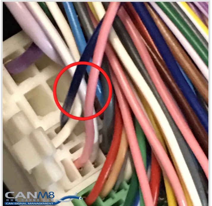
CAN Wires CAN HI = BLUE CAN LO = PINK
